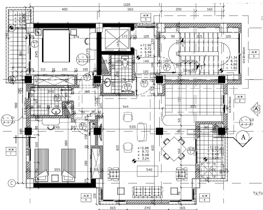
Typical Floor Plan_Type C
